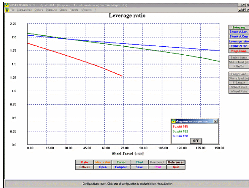
Suzuki GSX-R 1000 2004. "Leverage ratio" comparison diagram
